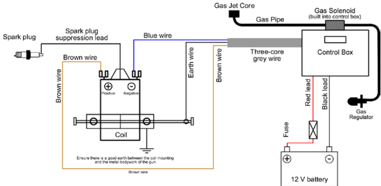
Figure 2. Retro-Fit Control Box Wiring Diagram
